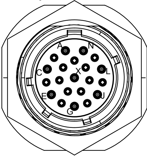
Front face of the optical transceiver insert shown, fiber optic cable plug opposite - see Appendix A2 for details
