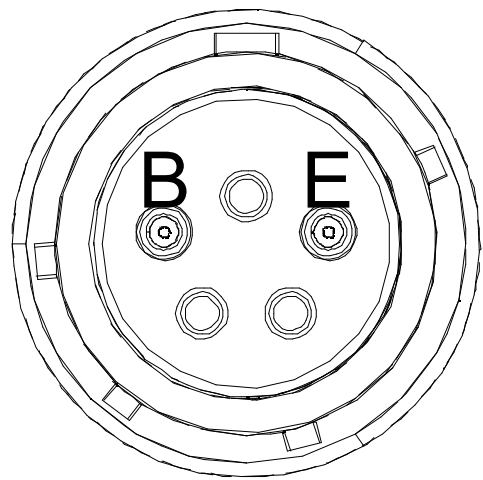
Front view of the MIL-DTL-38999 optical insert shown, fiber optic cable plug opposite - see Appendix A1 for mating connector details.
