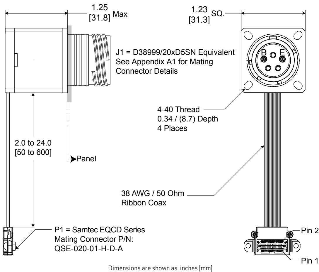
OUTLINE DRAWING - FLANGE OPTION
