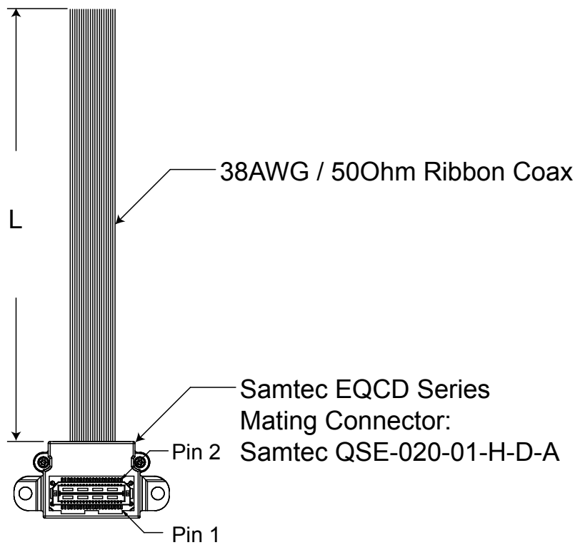
OUTLINE DRAWING CABLE LENGTH OPTIONS
