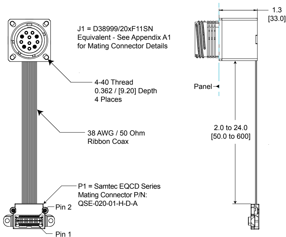
OUTLINE DRAWING - FLANGE MOUNTING OPTION
