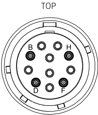
Front view of the D38999 optical insert shown, fiber optic cable plug opposite - see Appendix A1 for mating connector details.
