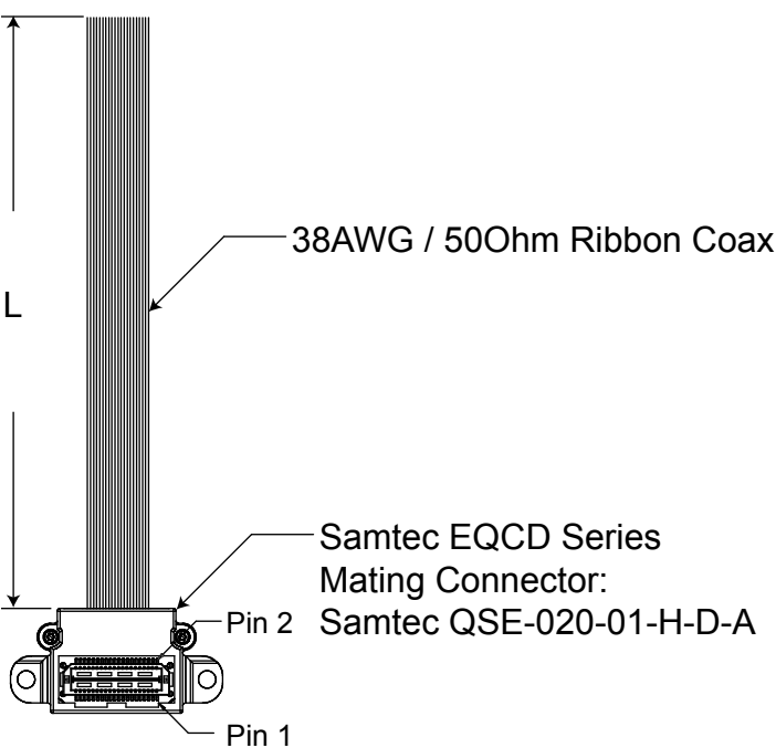
OUTLINE DRAWING CABLE LENGTH OPTIONS
