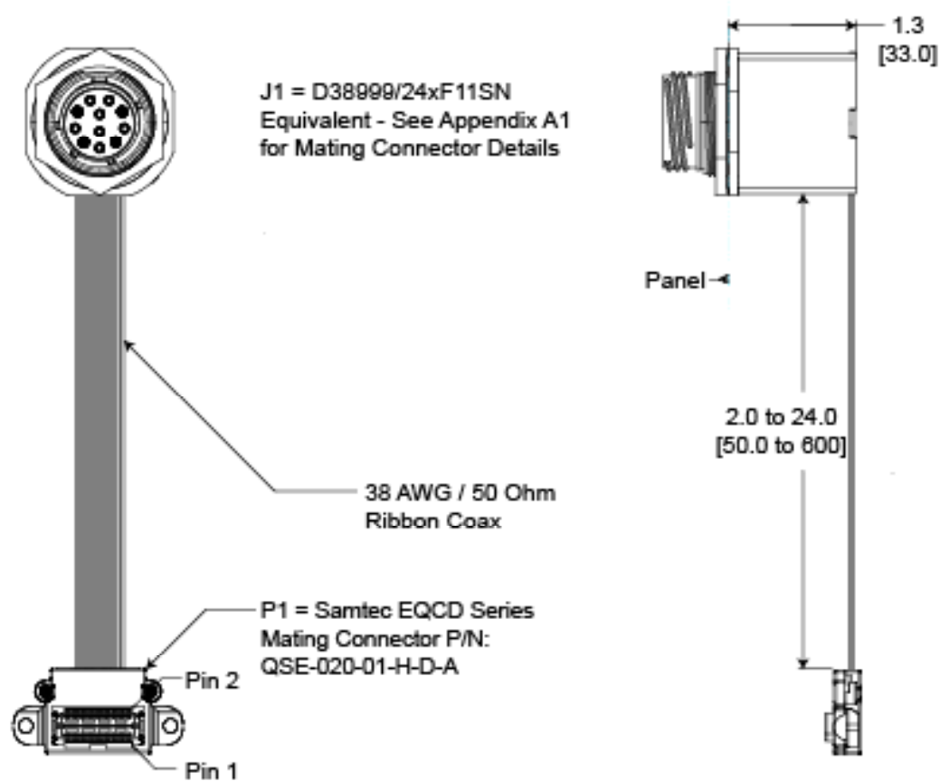
OUTLINE DRAWING - JAM NUT OPTION
