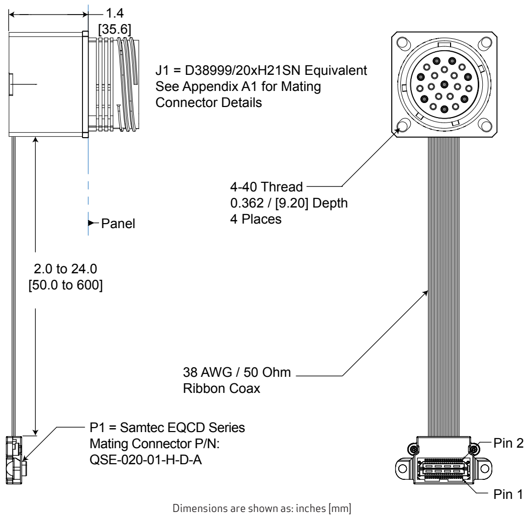
PANEL CUTOUT DIMENSIONS REAR PANEL MOUNTING ONLY
