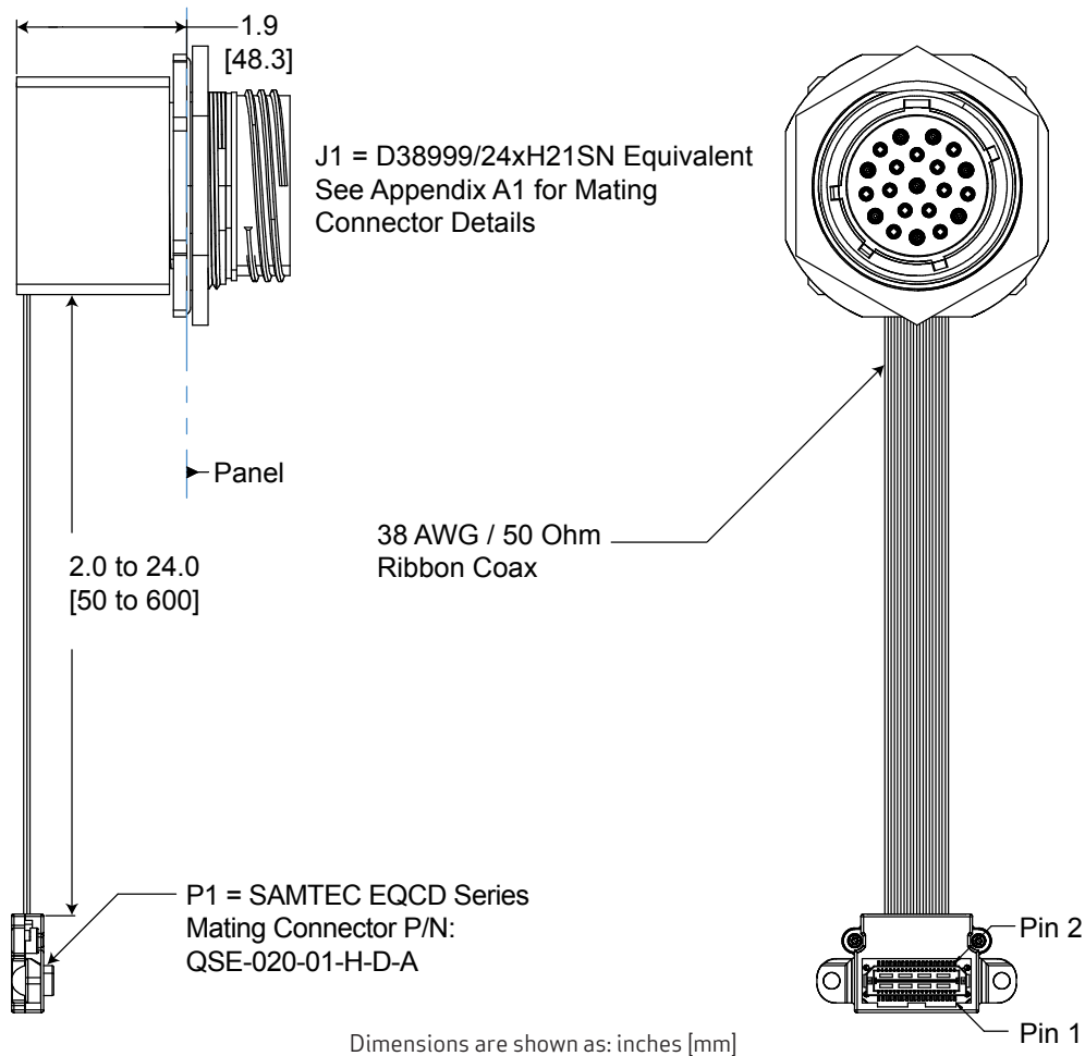
OUTLINE DRAWING - JAM NUT OPTION
